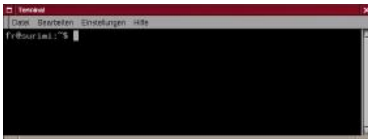
Abbildung 5-33. WindowMaker
